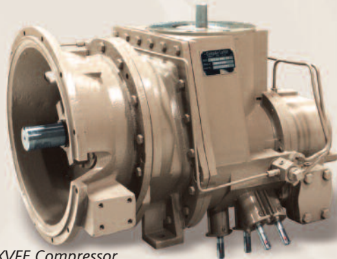
HG17XXXVFE Compressor with Bell Housing and Versatrol
